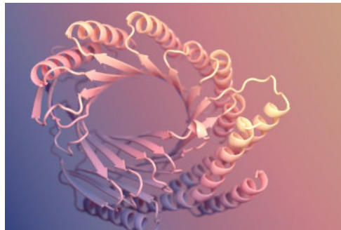
AlphaFold3
